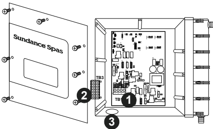
Figure C Terminal Block 240V Wire Connection
