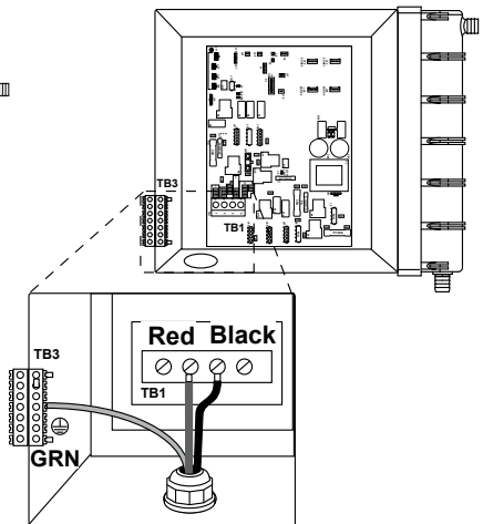
Figure D Control Box
